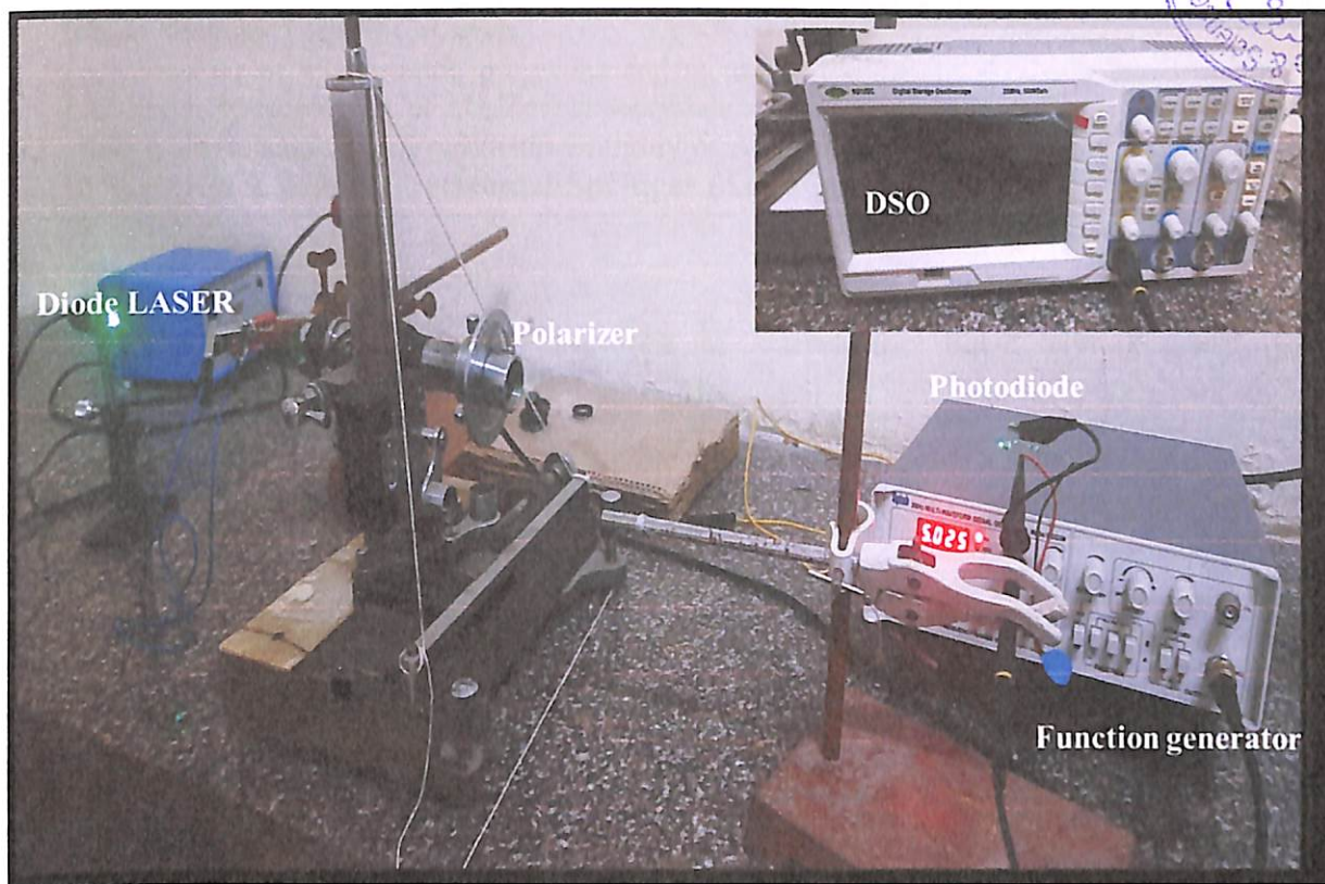
Figure 2: Photograph of response time measurement setup
